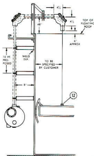
CAT. NO. 43100A FLOATING ROOF TANK
