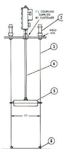
CAT. NO. 42100A TANK TOP READING GAUGE
