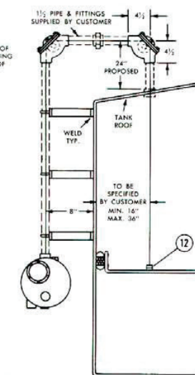
CAT. NO. 43400A FLOATING ROOF TANK UNDER FIXED ROOF
