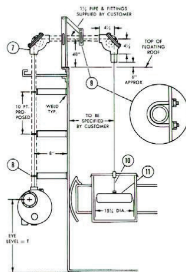
CAT. NO. 43000A FLOATING ROOF TANK FLOAT WELL
