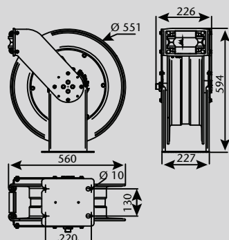
Dimensions (mm)
